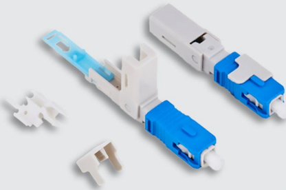
LX-DR12-B(52mm)-UPC
