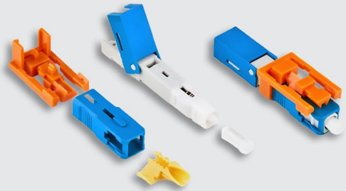
LX-14(52mm)-UPC
