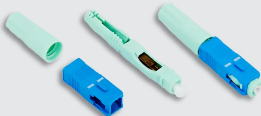
LX-R03(53mm)-UPC
