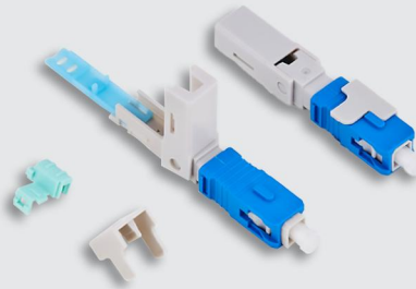
LX-DR12-A(52mm)-UPC
