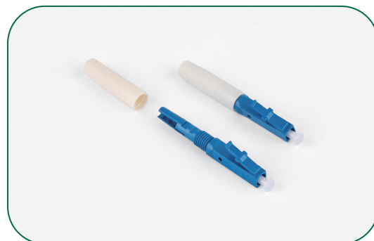
LX-LC-D(45mm)-通用型(GENERAL TYPE)-UPC
